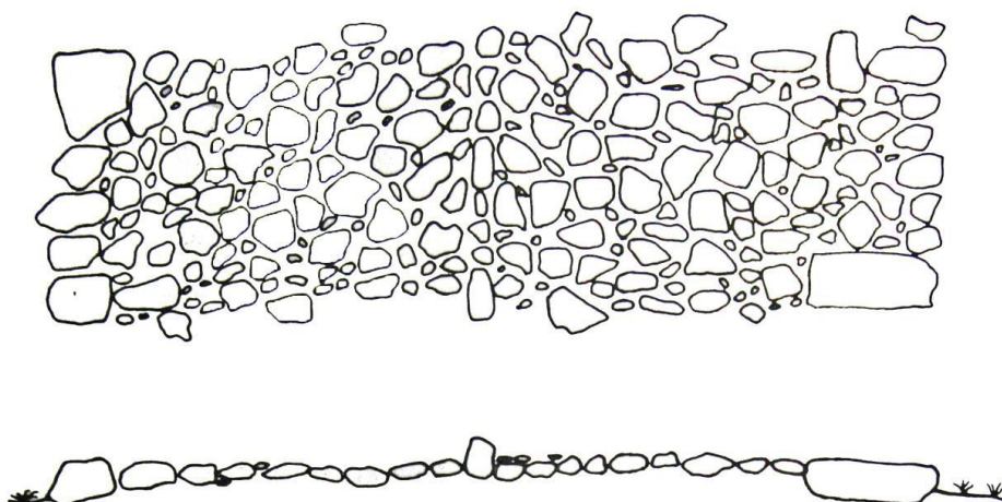
Fig. 2. Technique for Plain Terrains (French, 1981)
