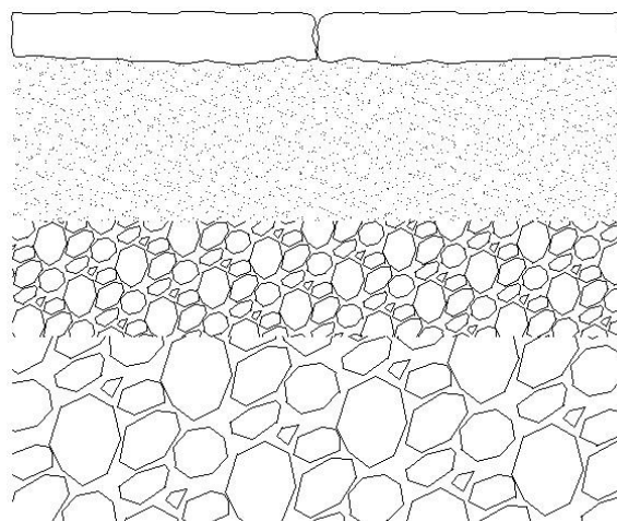
Fig. 1. Section of Roman Road
