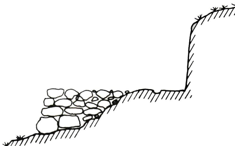
Fig. 4. Technique for Main Rock is Carved (French, 1981)
